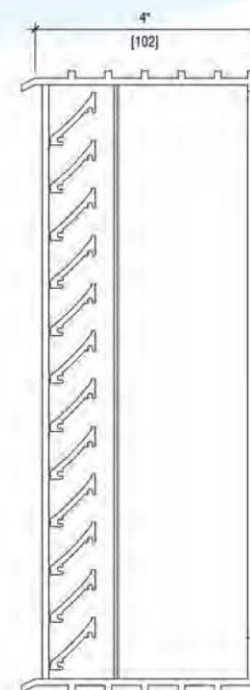
VERTICAL SECTION
