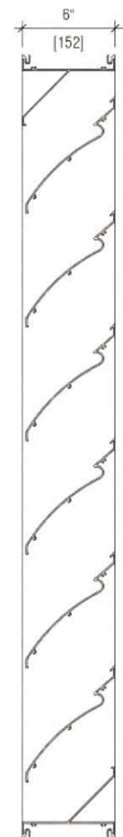
VERTICAL SECTION
